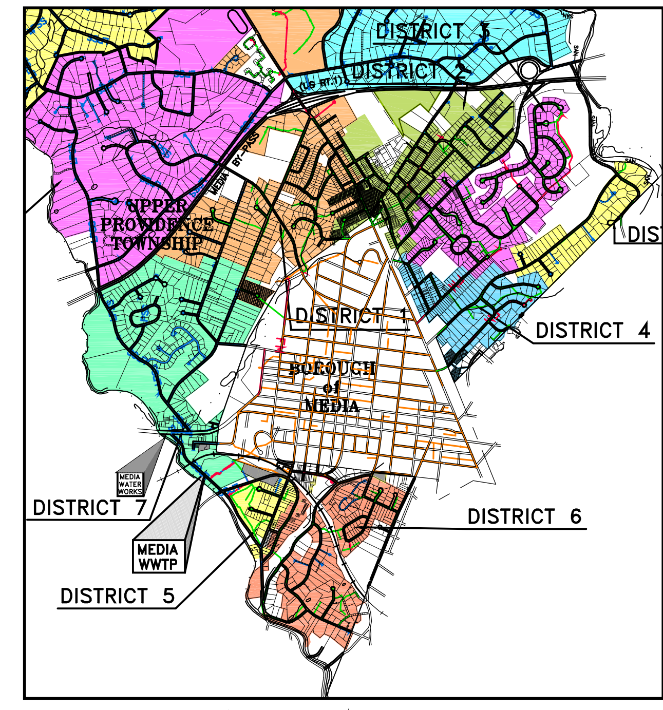
SANITARY SEWER DISTRICT LOCATION MAP SCALE: 1" = 2,000'
